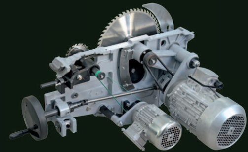
Complete mechanics + scoring unit 0.75 kW Komplette Mechanik + Vorritzer 0.75 kW
